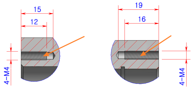
"상세뷰 C ( 1 : 1 )"
