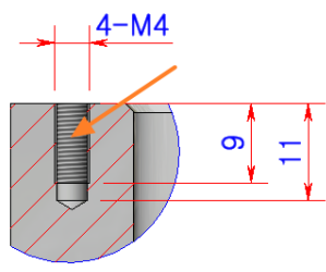
"상세뷰 E ( 1 : 1 )"
