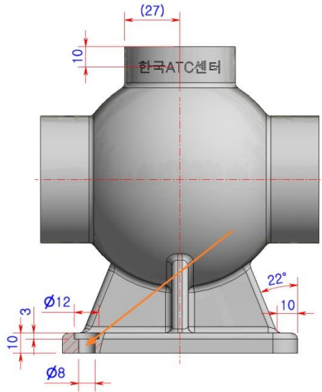
"상세뷰 E ( 1 : 1 )"
