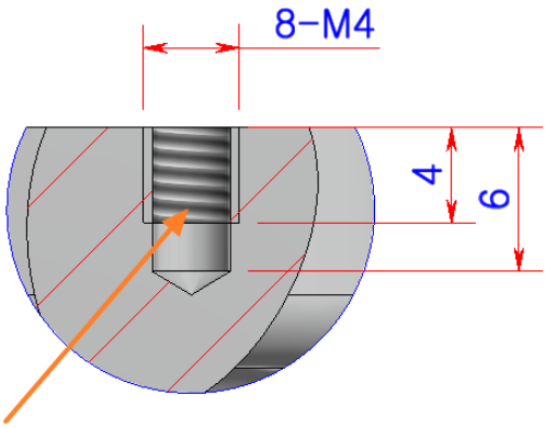
"상세뷰 D (2:1)"
