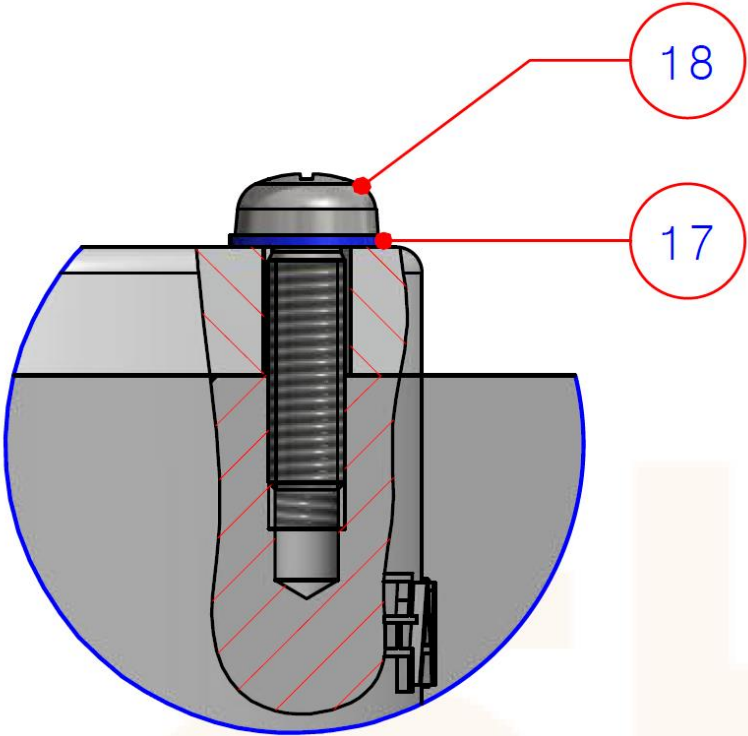
"상세뷰 D (2:1)"
