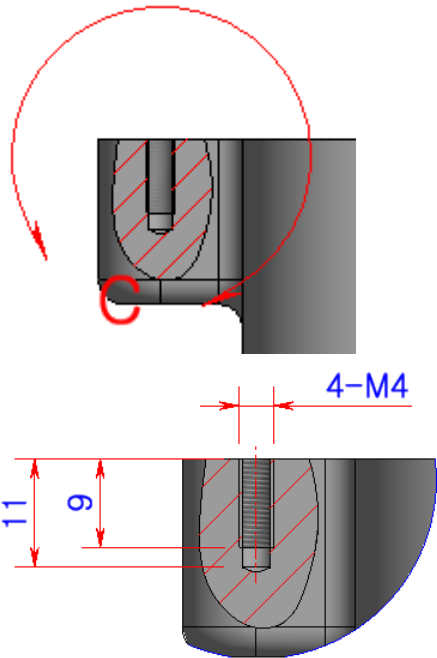
"상세뷰C(1:1)"
