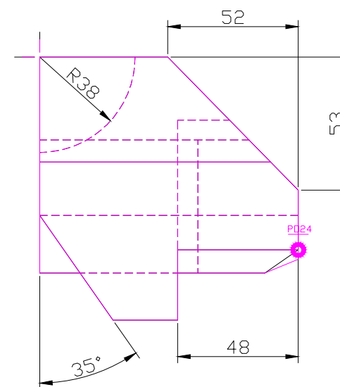
RIGHT SCALE 1/2
