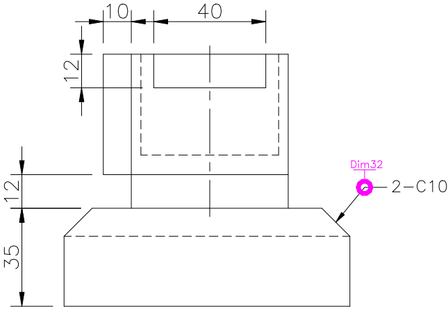
RIGHT SCALE 1/2
