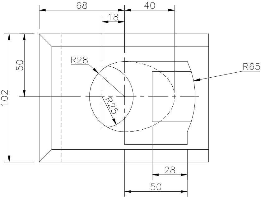
TOP SCALE 1/2
