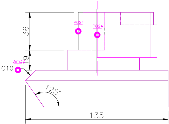
FRONT SCALE 1/2
