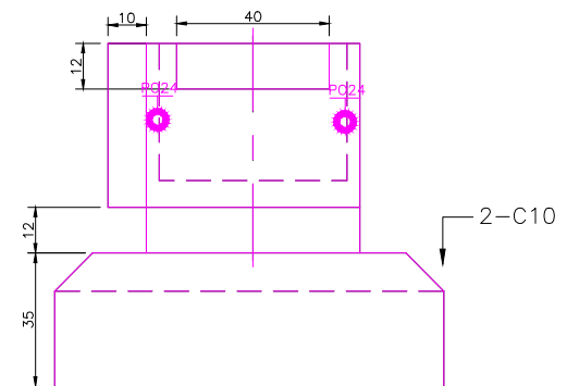
RIGHT
