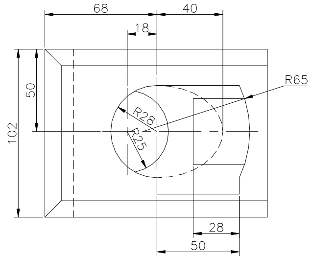
TOP SCALE 1/2
