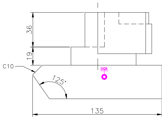
FRONT SCALE 1/2
