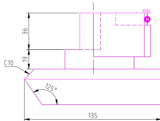
FRONT SCALE 1/2
