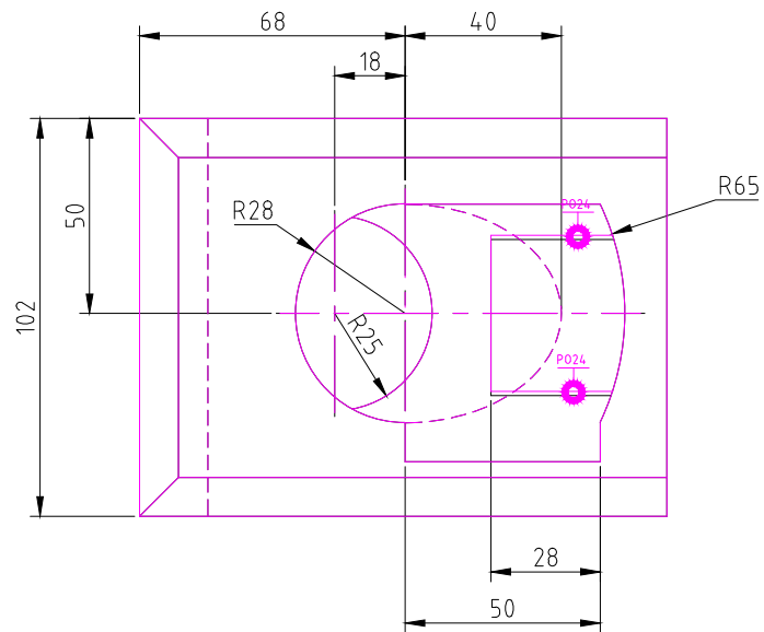
TOP SCALE 1/2
