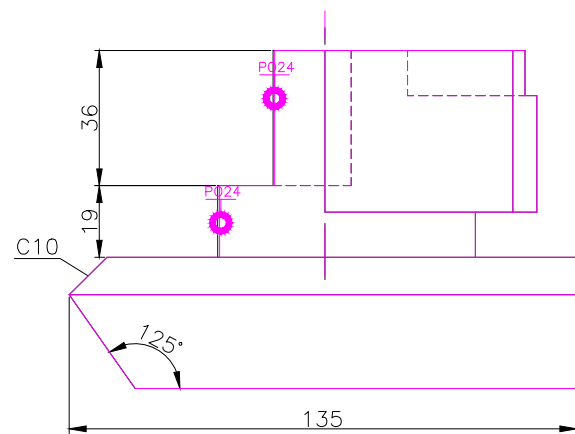
FRONT SCALE 1/2
