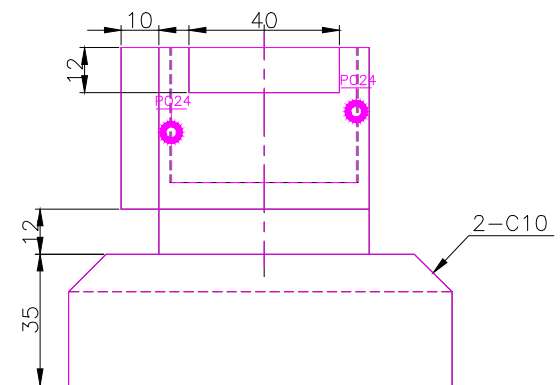
RIGHT SCALE 1/2
