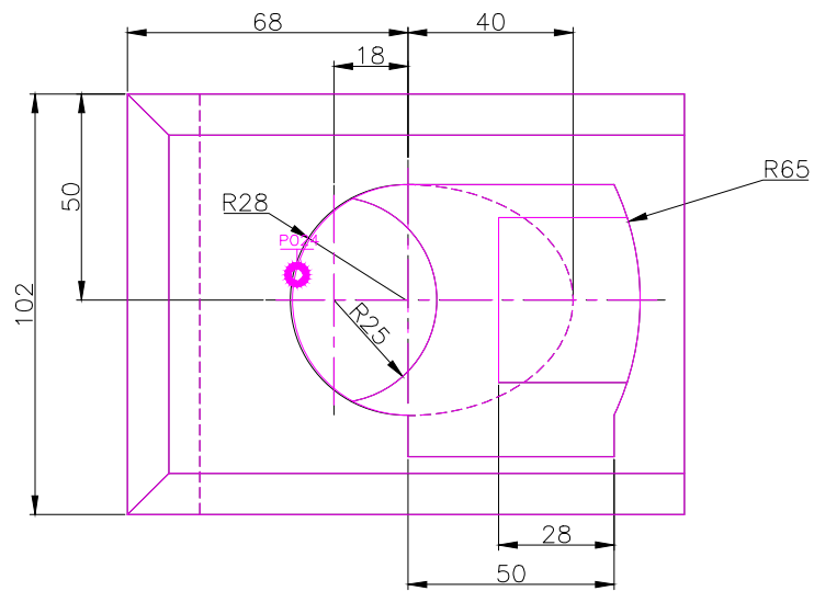
TOP SCALE 1/2
