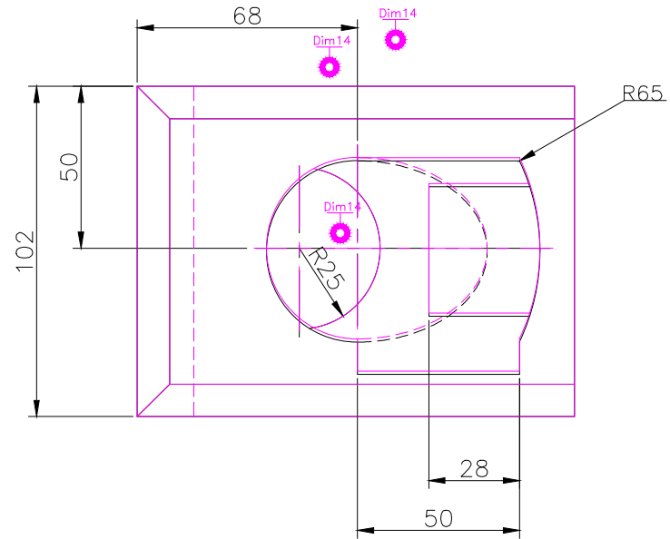
TOP SCALE 1/2
