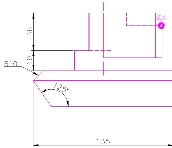
FRONT SCALE 1/2
