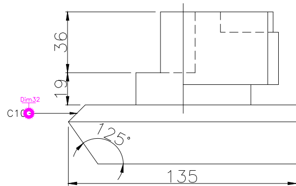
FRONT SCALE 1/2
