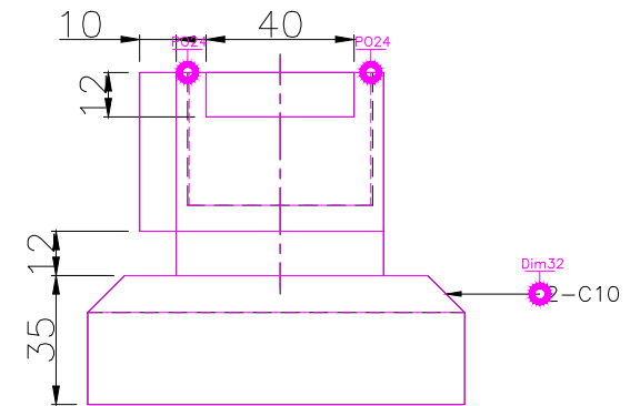
RIGHT SCALE 1/2
