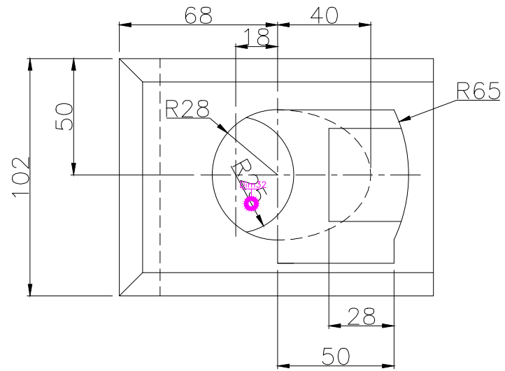
TOP SCALE 1/2
