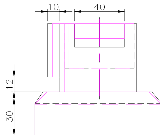
RIGHT SCALE 1/2
