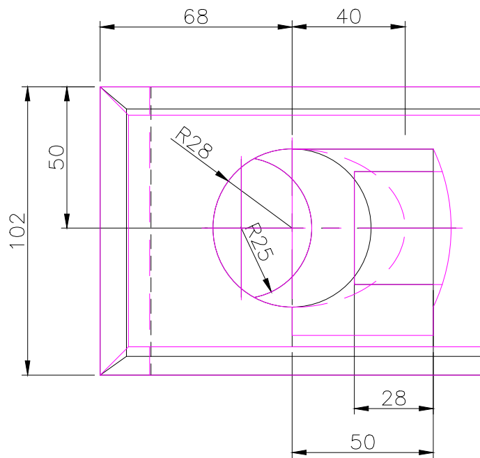
TOP SCALE 1/2
