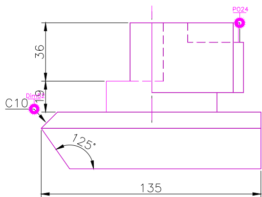
FRONT SCALE 1/2
