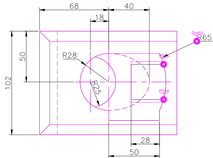
TOP SCALE 1/2
