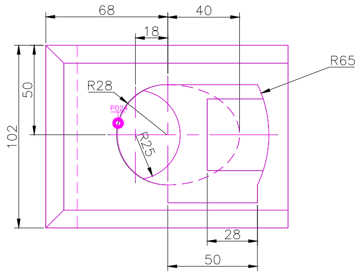
TOP SCALE 1/2
