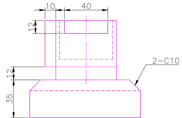
RIGHT SCALE 1/2
