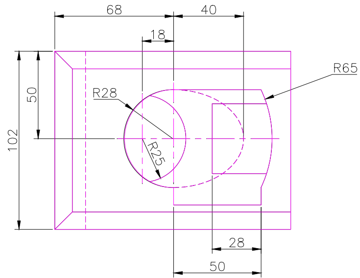
TOP SCALE 1/2
