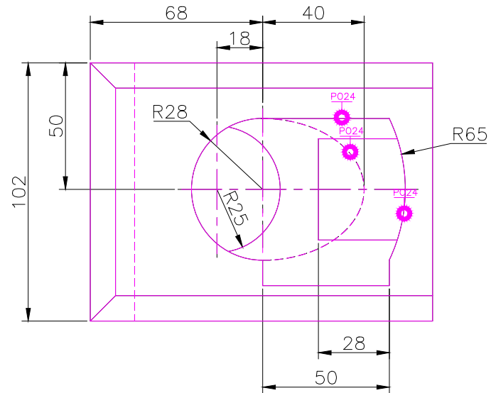
TOP SCALE 1/2
