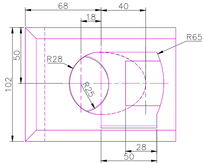
TOP SCALE 1/2
