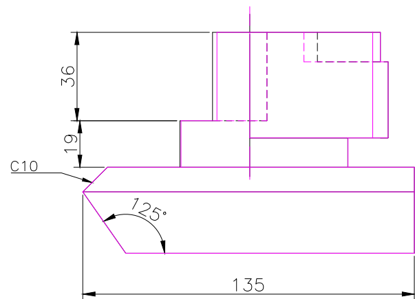
FRONT SCALE 1/2
