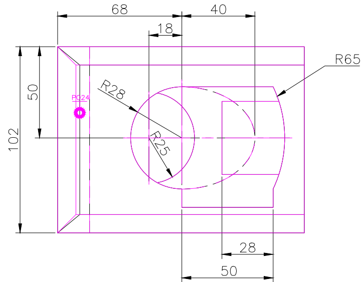
TOP SCALE 1/2
