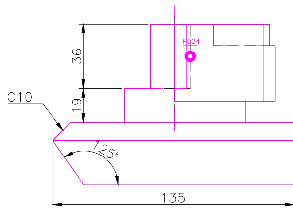
FRONT SCALE 1/2
