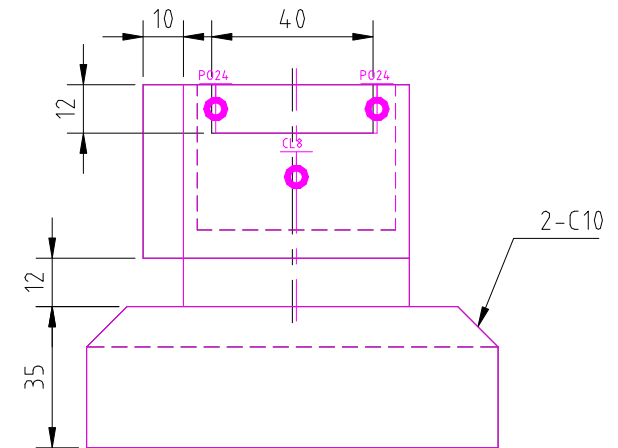
RIGHT SCALE 1/2
