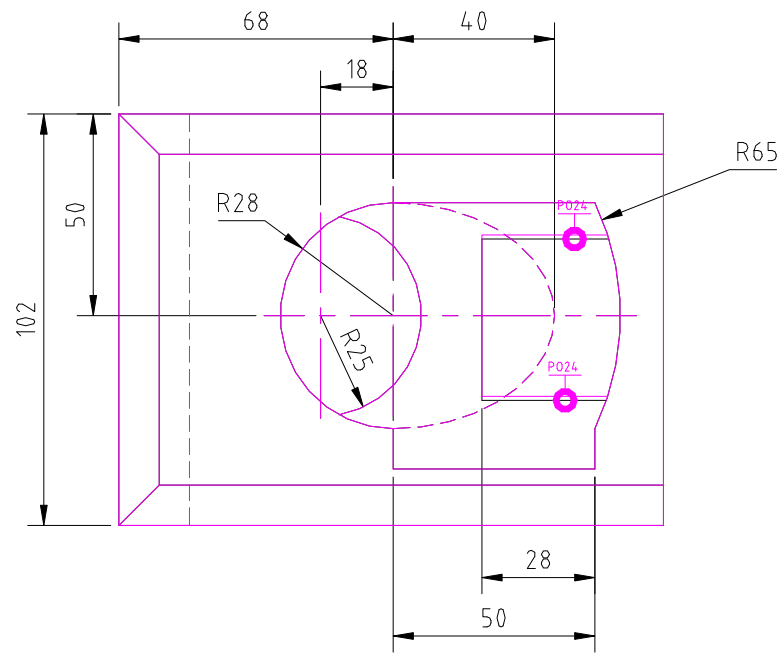
TOP SCALE 1/2
