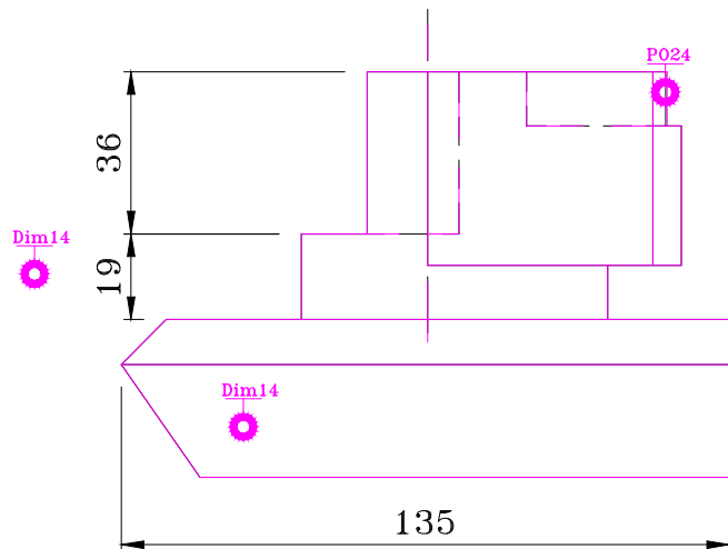
TOP SCALE 1/2
