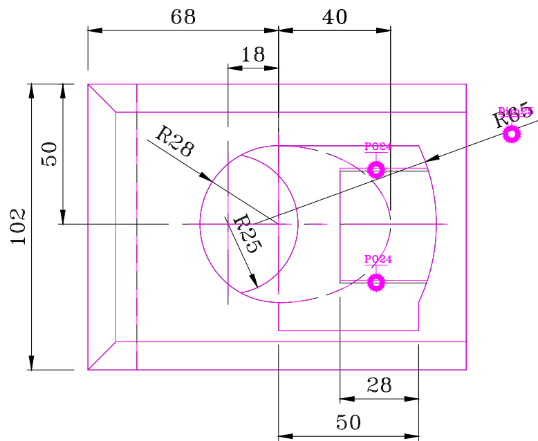
TOP SCALE 1/2
