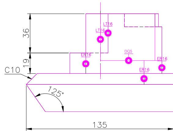
FRONT SCALE 1/2
