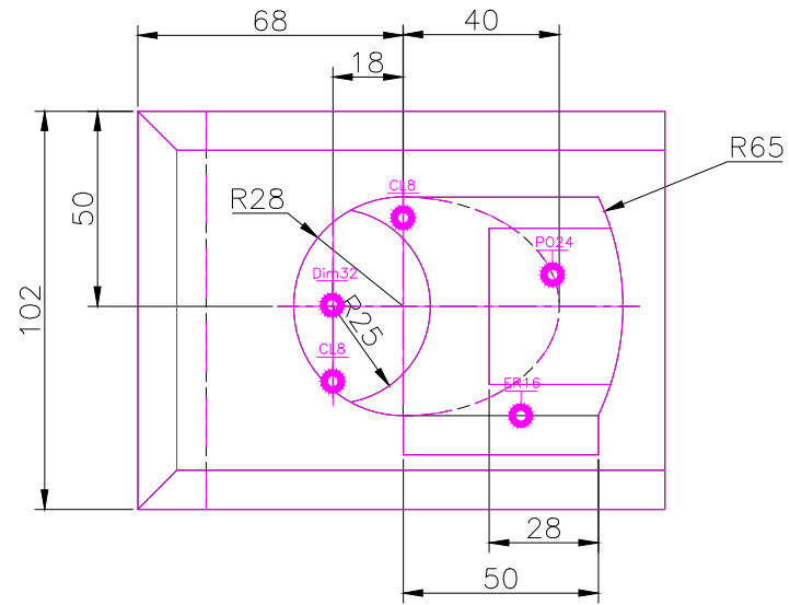
TOP SCALE 1/2
