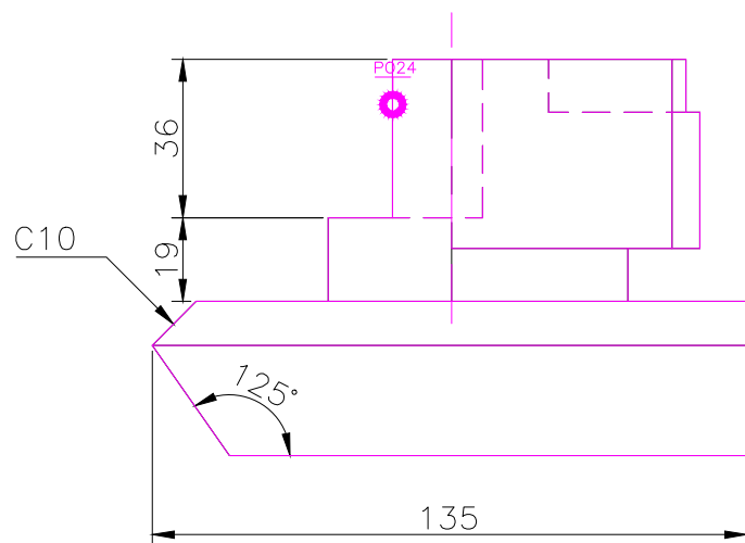
FRONT SCALE 1/2
