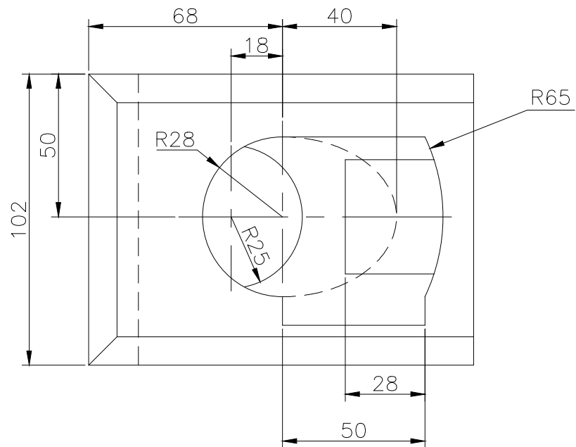
TOP SCALE 1/2
