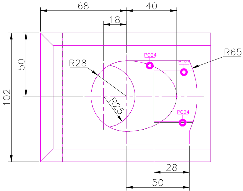
TOP SCALE 1/2
