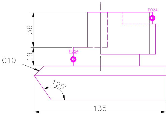
FRONT SCALE 1/2
