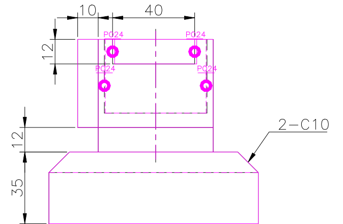
RIGHT SCALE 1/2
