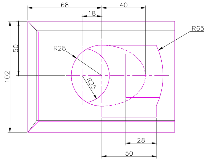
TOP SCALE 1/2
