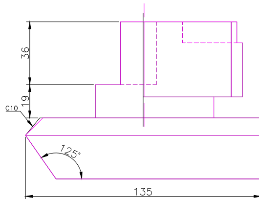
FRONT SCALE 1/2
