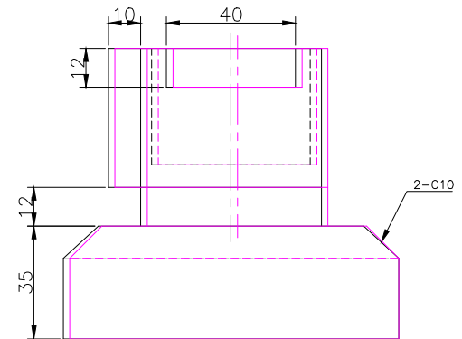
RIGHT SCALE 1/2
