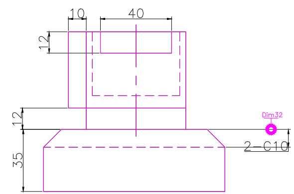
RIGHT SCALE 1/2
