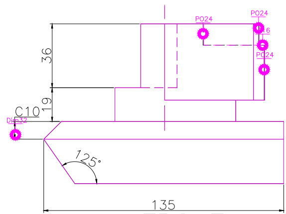
FRONT SCALE 1/2
