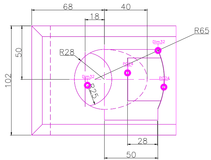
Top SCALE 1/2
