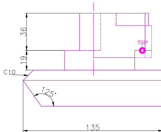
FRONT SCALE 1/2
