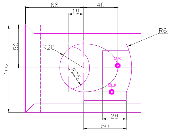
TOP SCALE 1/2
