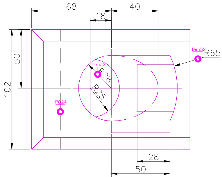
TOP SCALE 1/2
