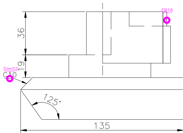
FRONT SCALE 1/2
