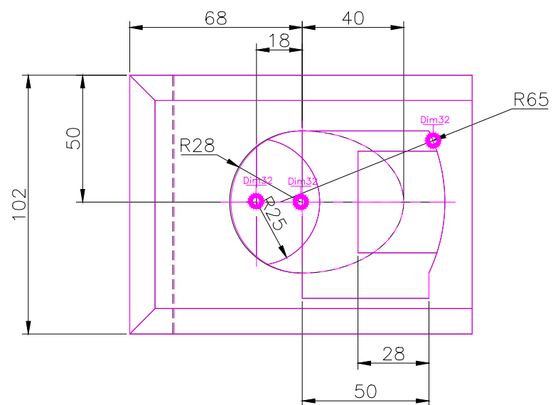
TOP SCALE 1/2
