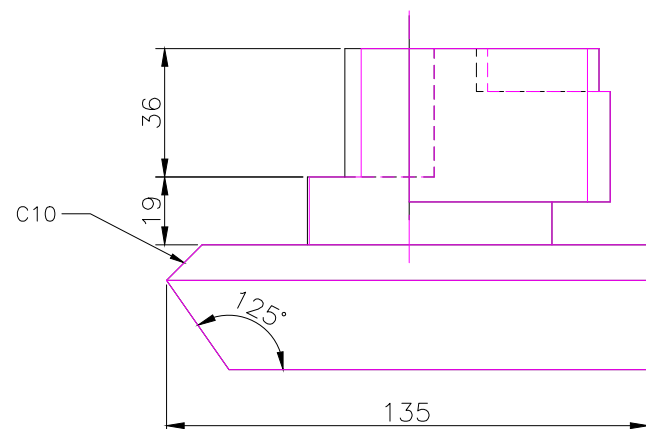
TOP SCALE 1/2
