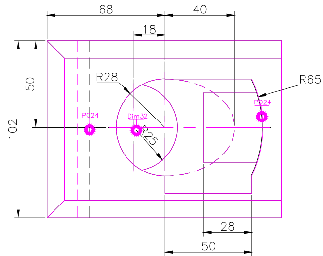
TOP SCALE 1/2
