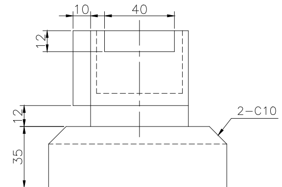
RIGHT SCALE 1/2
