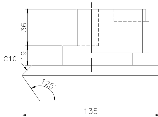
FRONT SCALE 1/2
