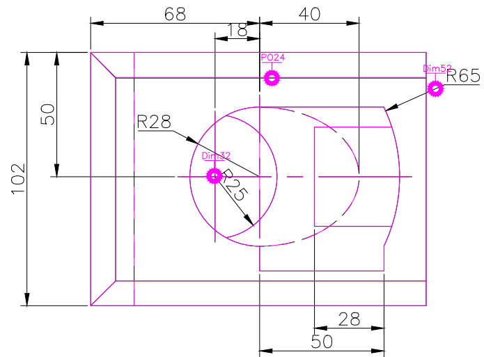
TOP SCALE 1/2
