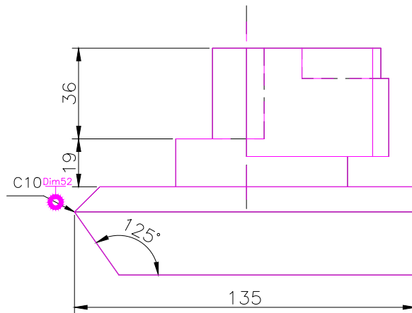
FRONT SCALE 1/2
