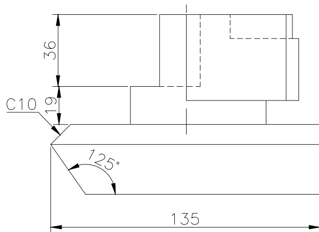
FRONT SCALE 1/2
