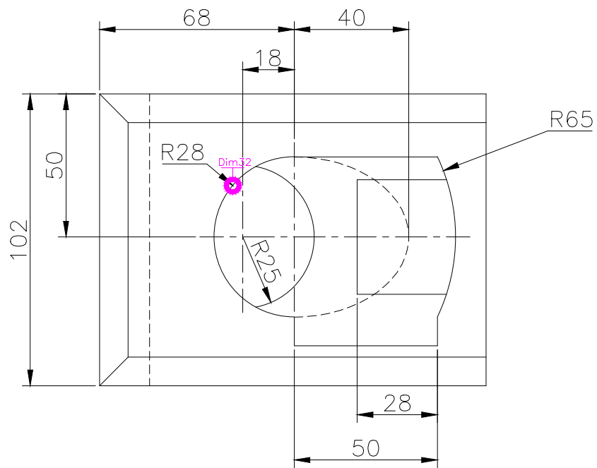
TOP SCALE 1/2
