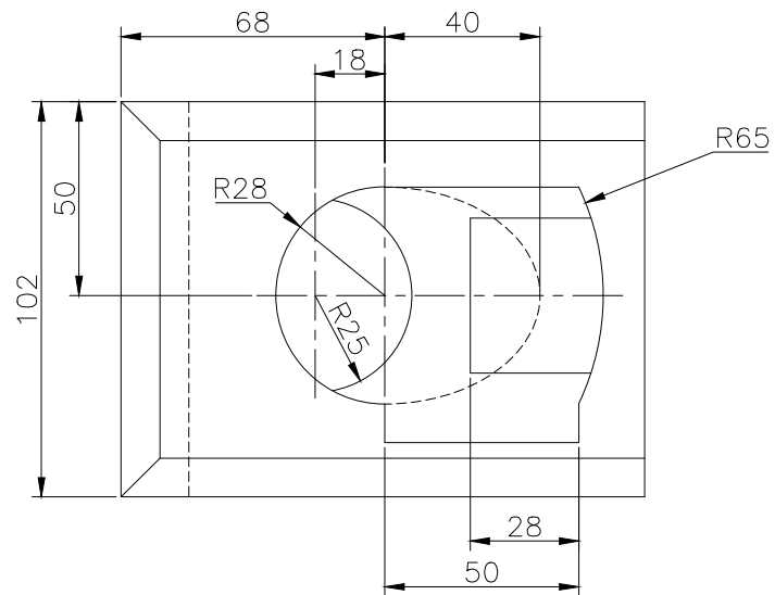
TOP SCALE 1/2
