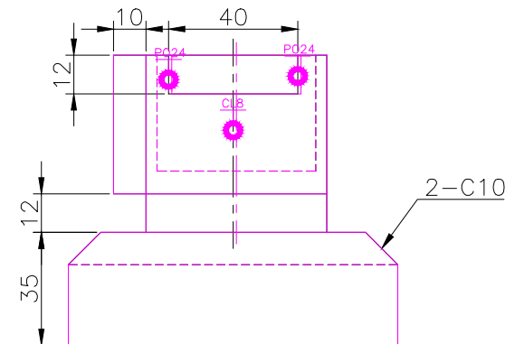
RIGHT SCALE 1/2
