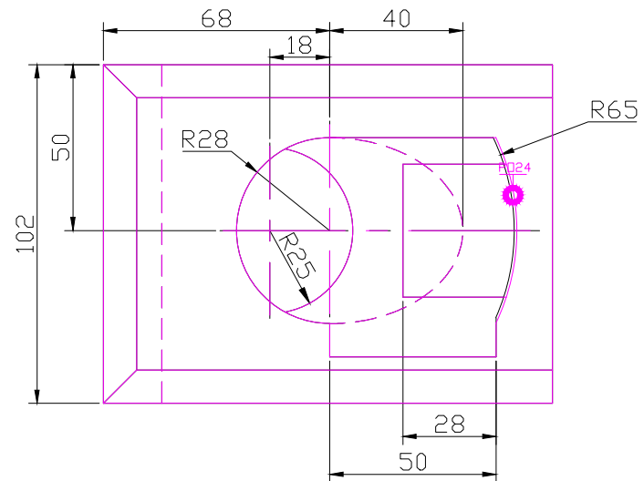
TOP SCALE 1/2
