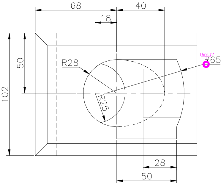
TOP SCALE 1/2
