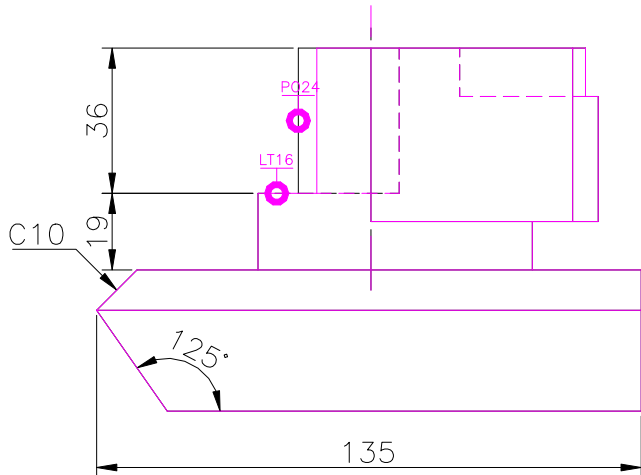
FRONT SCALE 1/2
