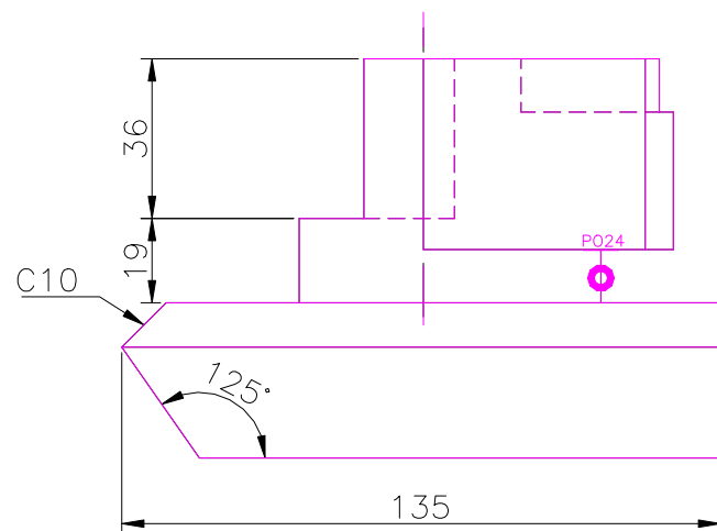
FRONT SCALE 1/2
