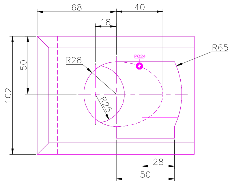
TOP SCALE 1/2
