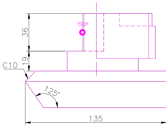
FRONT SCALE 1/2
