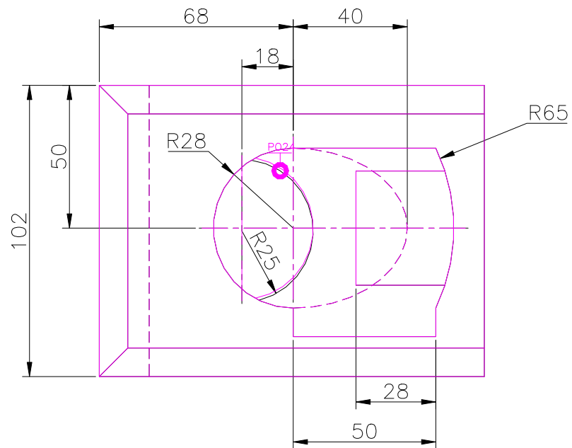
TOP SCALE 1/2
