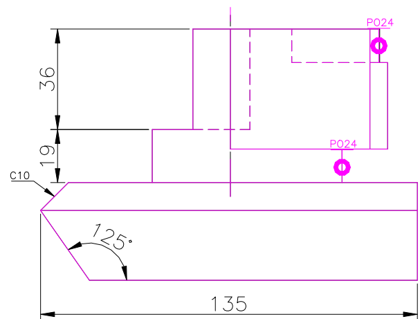
FRONT SCALE 1/2
