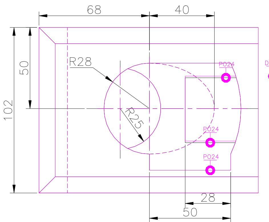
TOP SCALE 1/2
