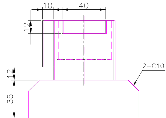
RIGHT SCALE 1/2
