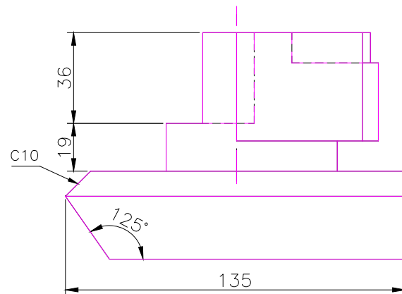
FRONT SCALE 1/2
