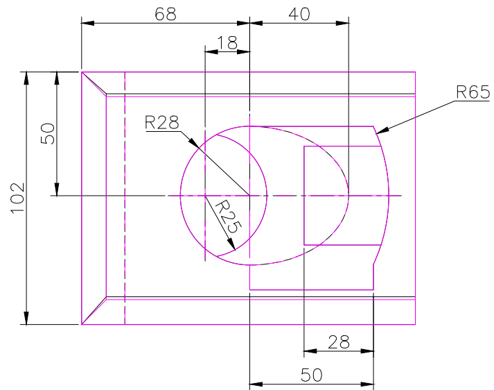
TOP SCALE 1/2
