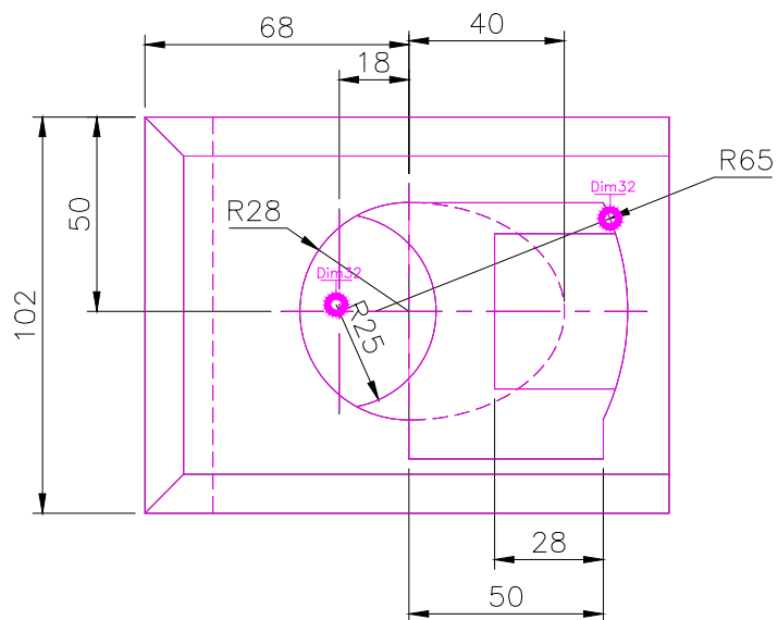
TOP SCALE 1/2
