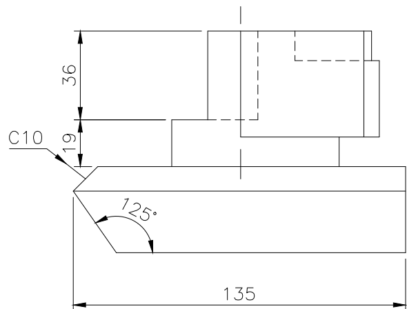
FRONT SCALE 1/2
