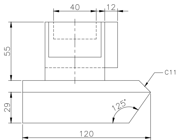
FRONT SCALE 1/2
