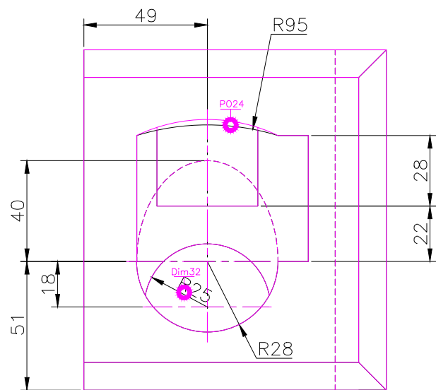
TOP SCALE 1/2
