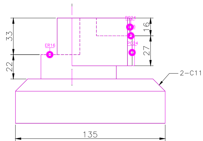
RIGHT SCALE 1/2
