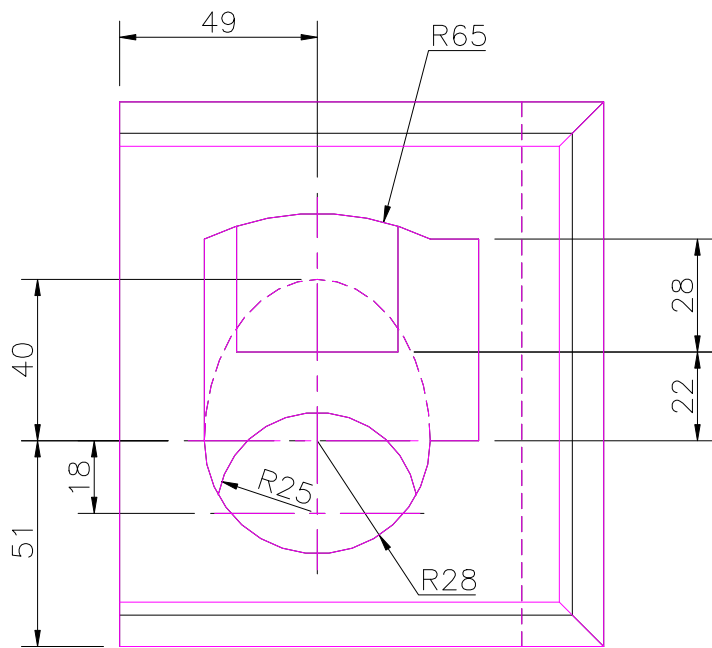
TOP SCALE 1/2
