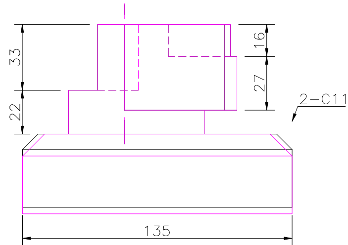
RIGHT SCALE 1/2
