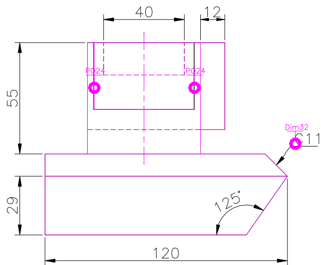
FRONT SCALE 1/2
