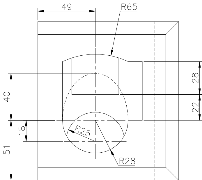
TOP SCALE 1/2
