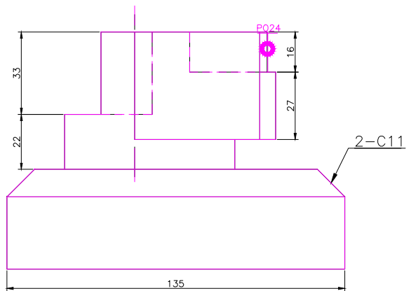
RIGHT SCALE 1/2
