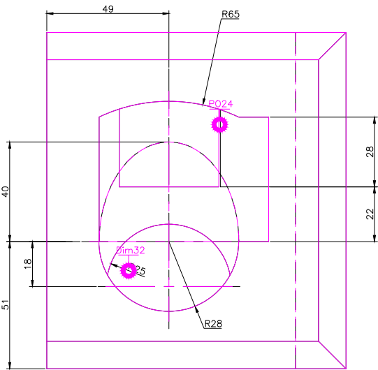
TOP SCALE 1/2
