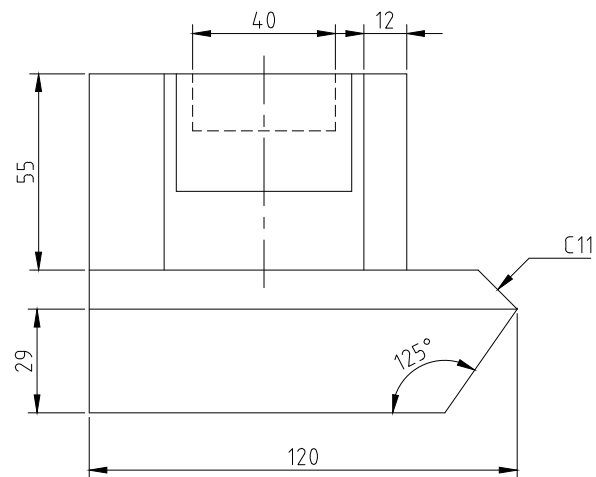
FRONT SCALE 1/2
