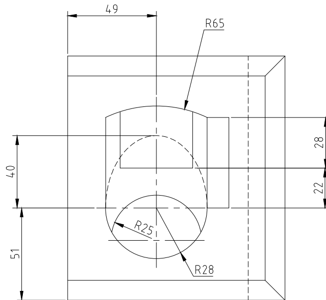
TOP SCALE 1/2
