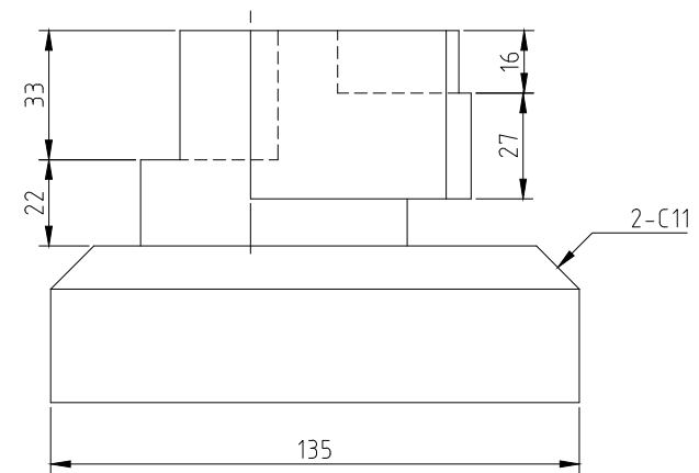
RIGHT SCALE 1/2
