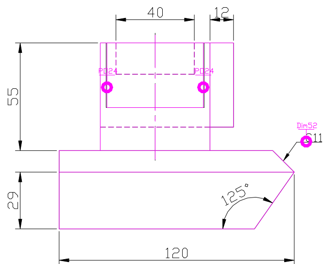
FRONT SCALE 1/2
