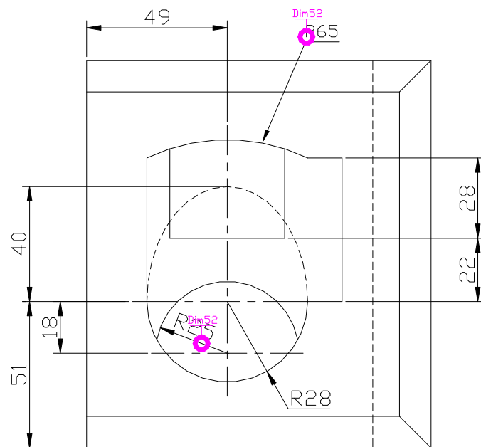
TOP SCALE 1/2
