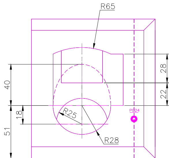
TOP SCALE 1/2
