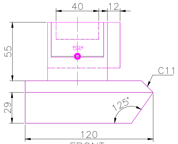
FRONT SCALE 1/2
