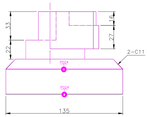
RIGHT SCALE 1/2
