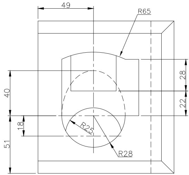
TOP SCALE 1/2
