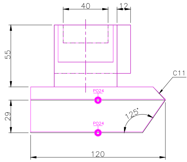
FRONT SCALE 1/2
